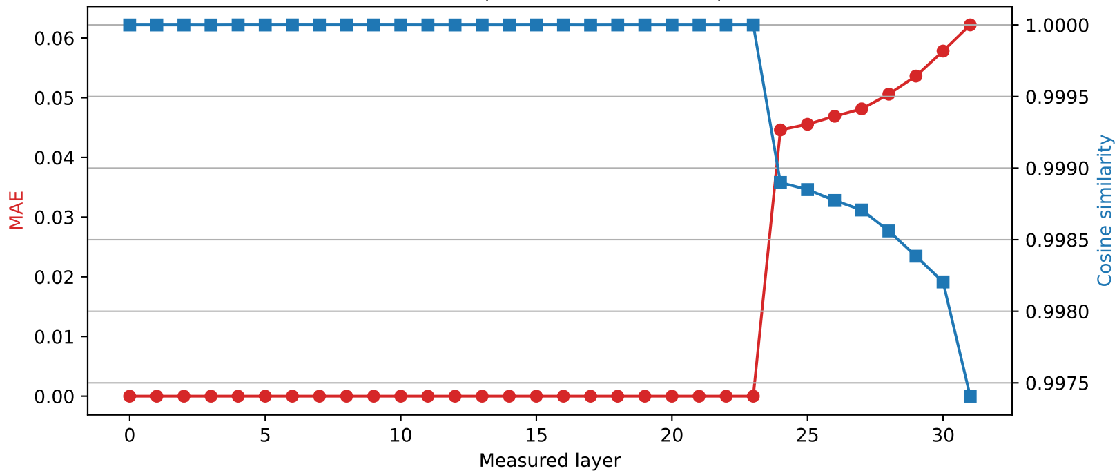
Mistral-7B-Instruct-v0.3 | Quantized layer 23 | float32 \rightarrow int4
