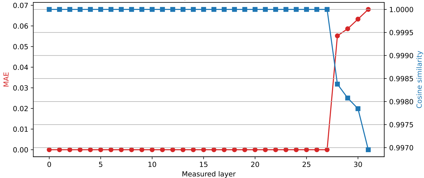
Mistral-7B-Instruct-v0.3 | Quantized layer 27 | float32 \rightarrow int4
