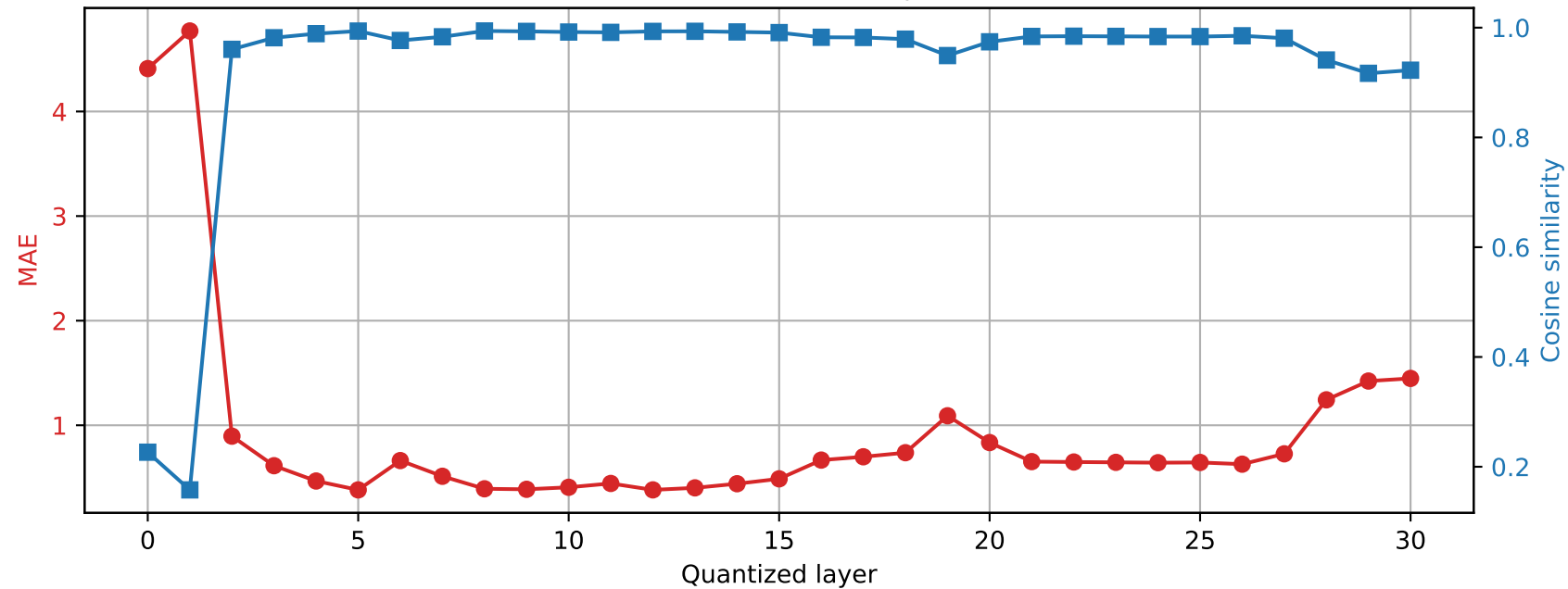
Mistral-7B-Instruct-v0.3 | Prompt 0 Final RMSNorm output damage | float32 → int2
