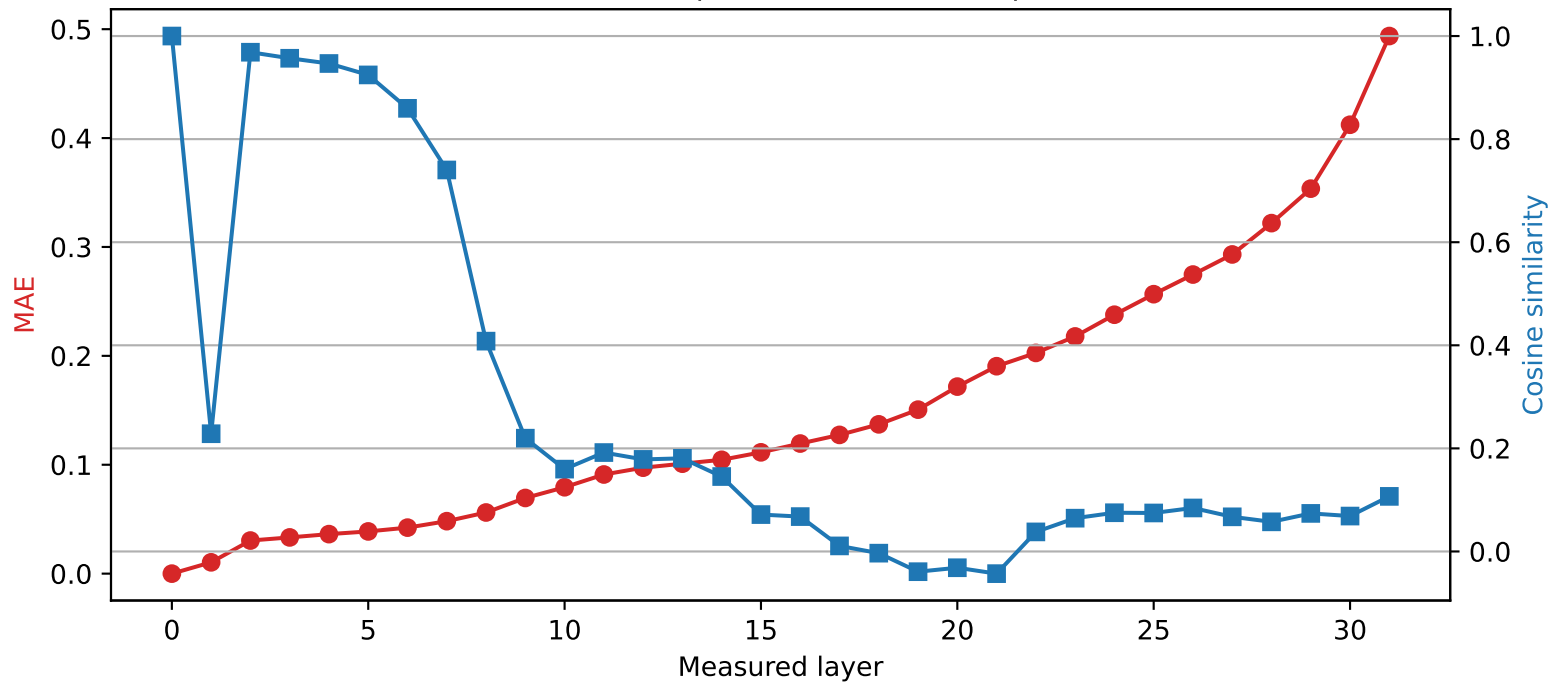
Mistral-7B-Instruct-v0.3 | Quantized layer 0 | float32 \rightarrow int2
