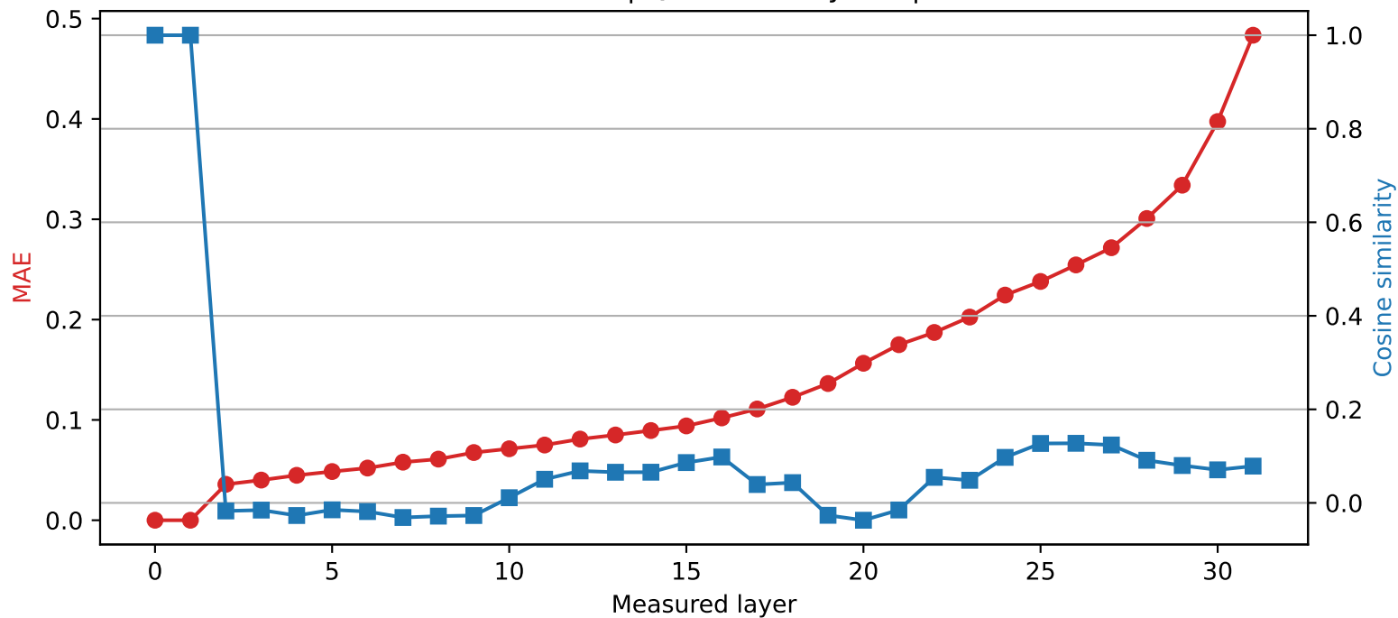
Mistral-7B-Instruct-v0.3 | Quantized layer 1 | float32 \rightarrow int2
