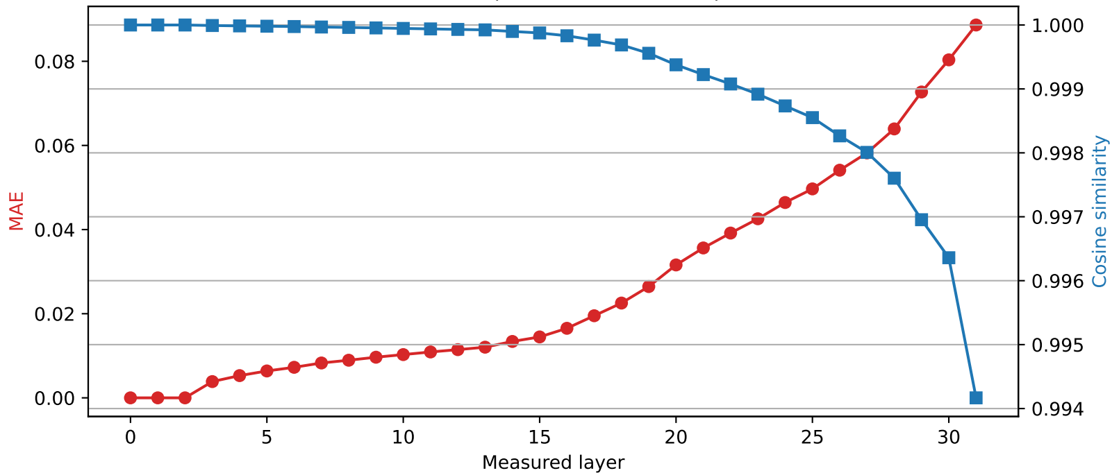
Mistral-7B-Instruct-v0.3 | Quantized layer 2 | float32 → int2
