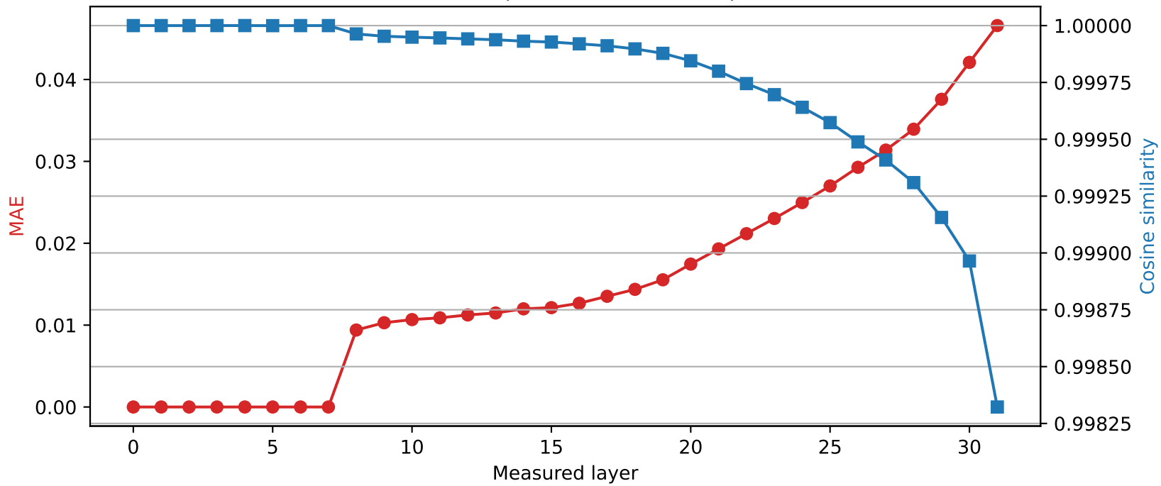
Mistral-7B-Instruct-v0.3 | Quantized layer 7 | float32 → int2
