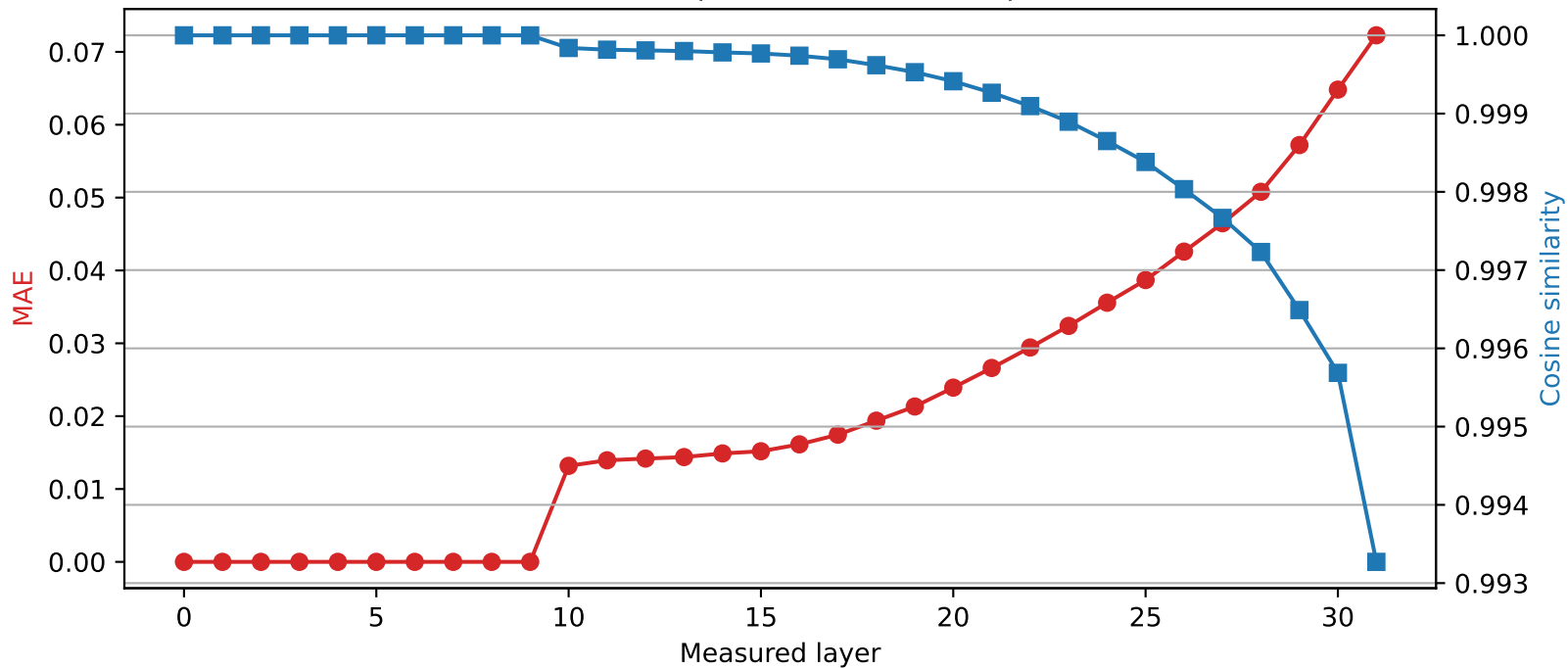
Mistral-7B-Instruct-v0.3 | Quantized layer 9 | float32 \rightarrow int2
