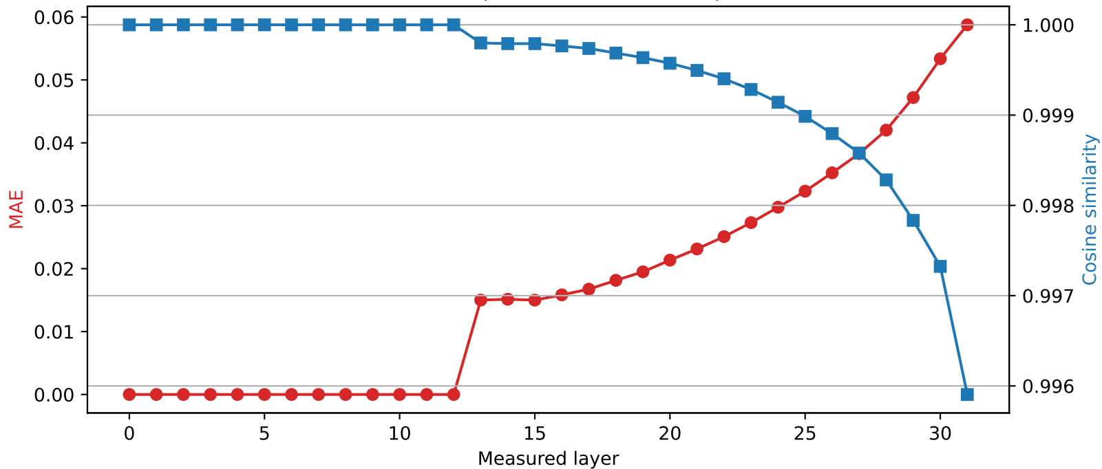
Mistral-7B-Instruct-v0.3 | Quantized layer 12 | float32 \rightarrow int2
