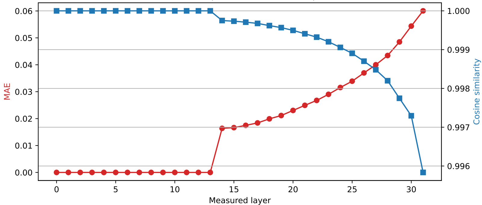
Mistral-7B-Instruct-v0.3 | Quantized layer 13 | float32 \rightarrow int2
