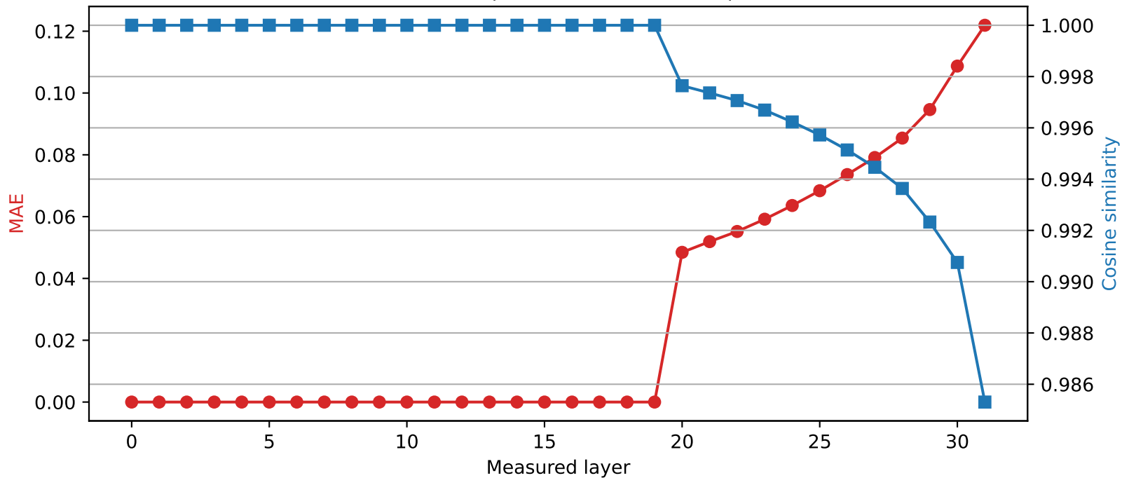
Mistral-7B-Instruct-v0.3 | Quantized layer 19 | float32 \rightarrow int2
