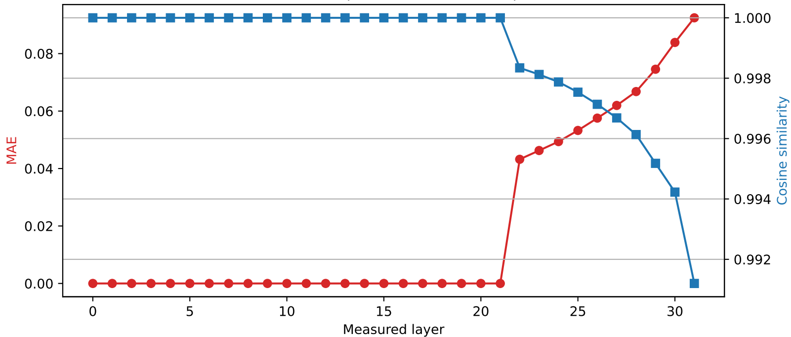
Mistral-7B-Instruct-v0.3 | Quantized layer 21 | float32 \rightarrow int2
