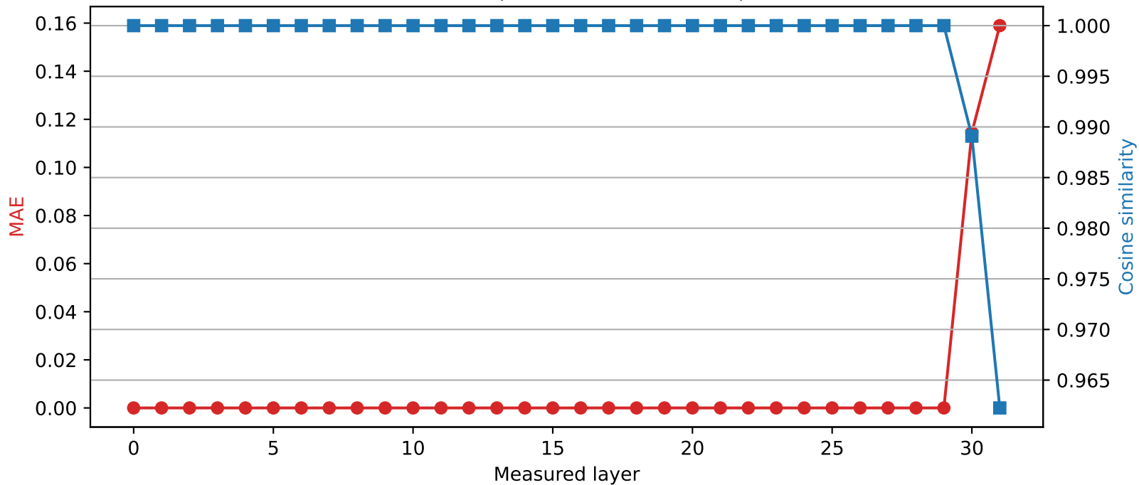
Mistral-7B-Instruct-v0.3 | Quantized layer 29 | float32 \rightarrow int2
