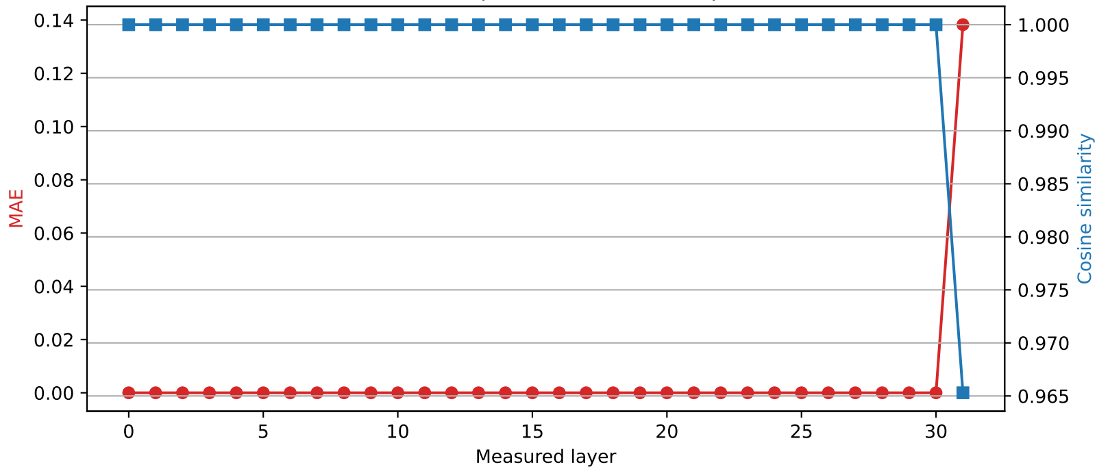
Mistral-7B-Instruct-v0.3 | Quantized layer 30 | float32 \rightarrow int2
