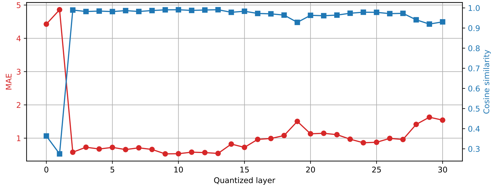
Mistral-7B-Instruct-v0.3 | Prompt 2 Final RMSNorm output damage | float32 \rightarrow int2
