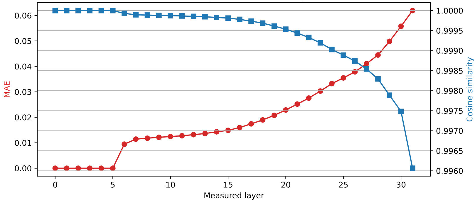
Mistral-7B-Instruct-v0.3 | Quantized layer 5 | float32 \rightarrow int2
