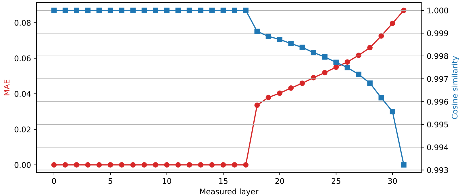
Mistral-7B-Instruct-v0.3 | Quantized layer 17 | float32 \rightarrow int2
