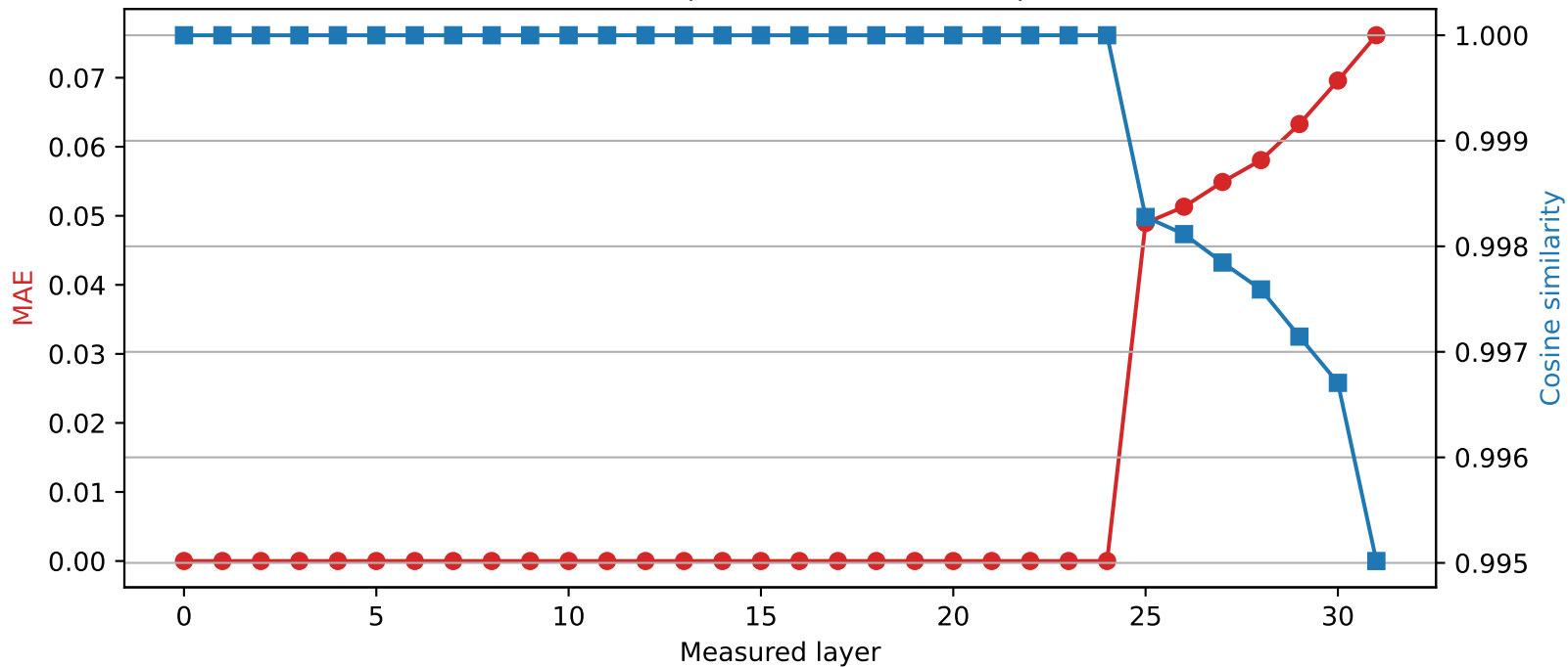
Mistral-7B-Instruct-v0.3 | Quantized layer 24 | float32 \rightarrow int2
