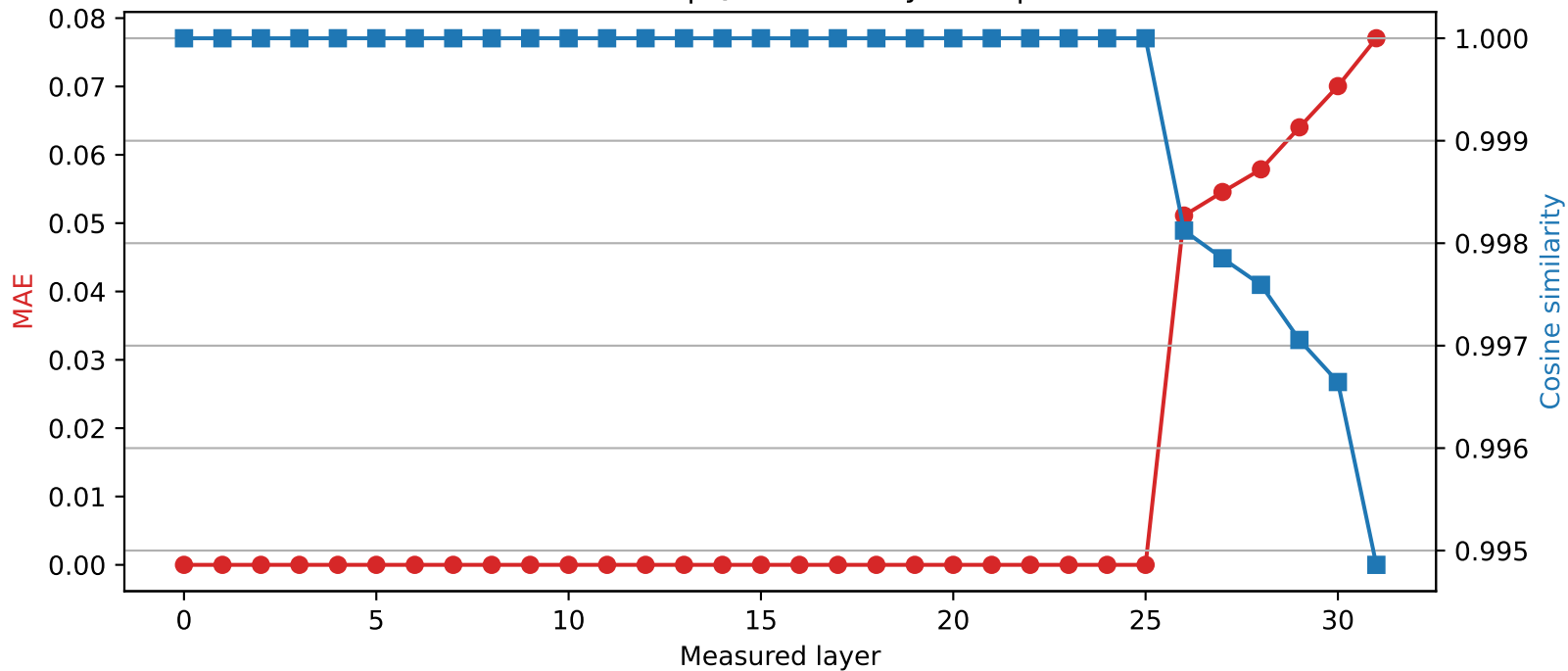
Mistral-7B-Instruct-v0.3 | Quantized layer 25 | float32 \rightarrow int2
