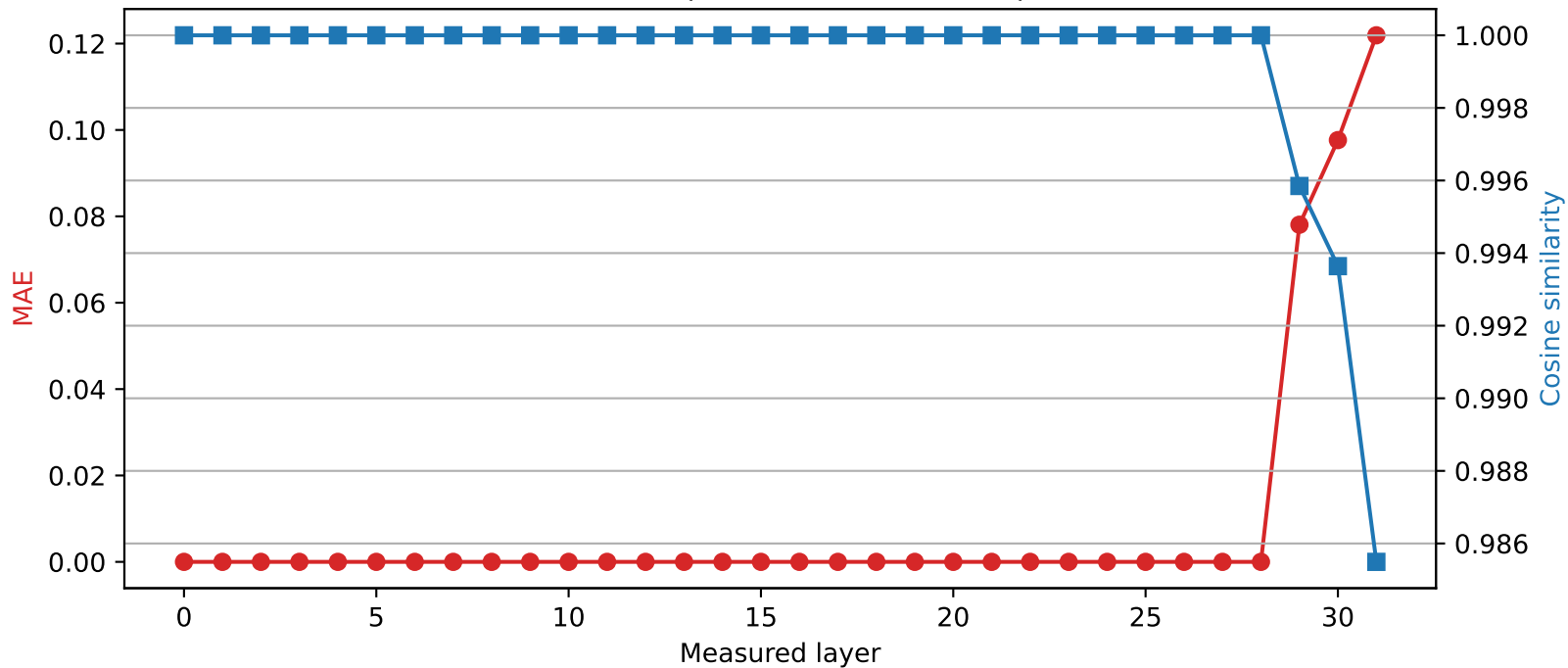
Mistral-7B-Instruct-v0.3 | Quantized layer 28 | float32 \rightarrow int2
