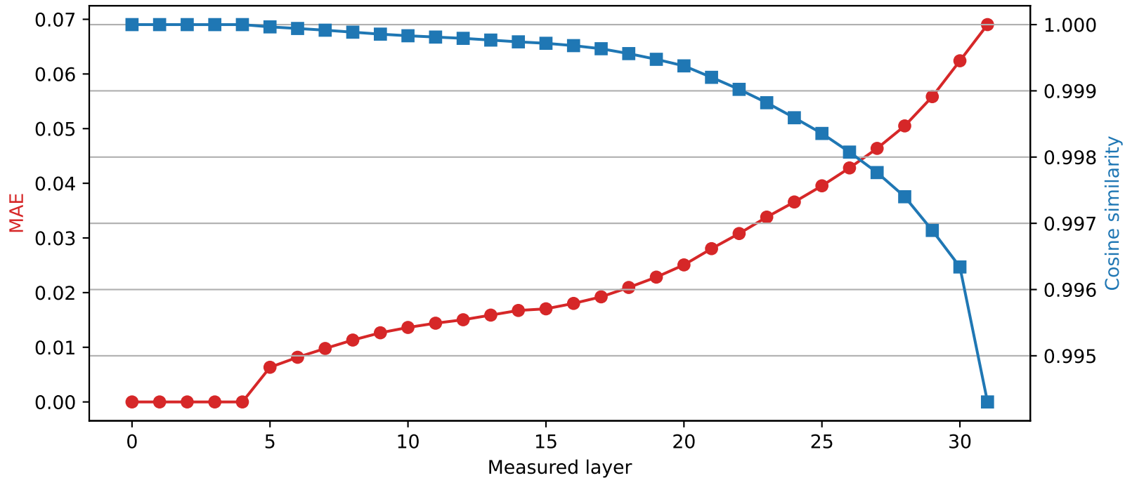
Mistral-7B-Instruct-v0.3 | Quantized layer 4 | float32 \rightarrow int2
