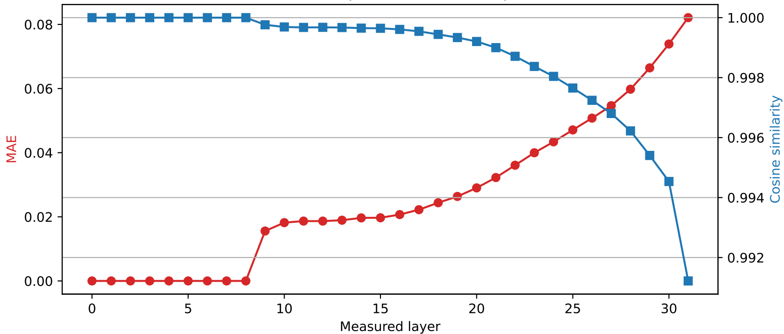
Mistral-7B-Instruct-v0.3 | Quantized layer 8 | float32 → int2
