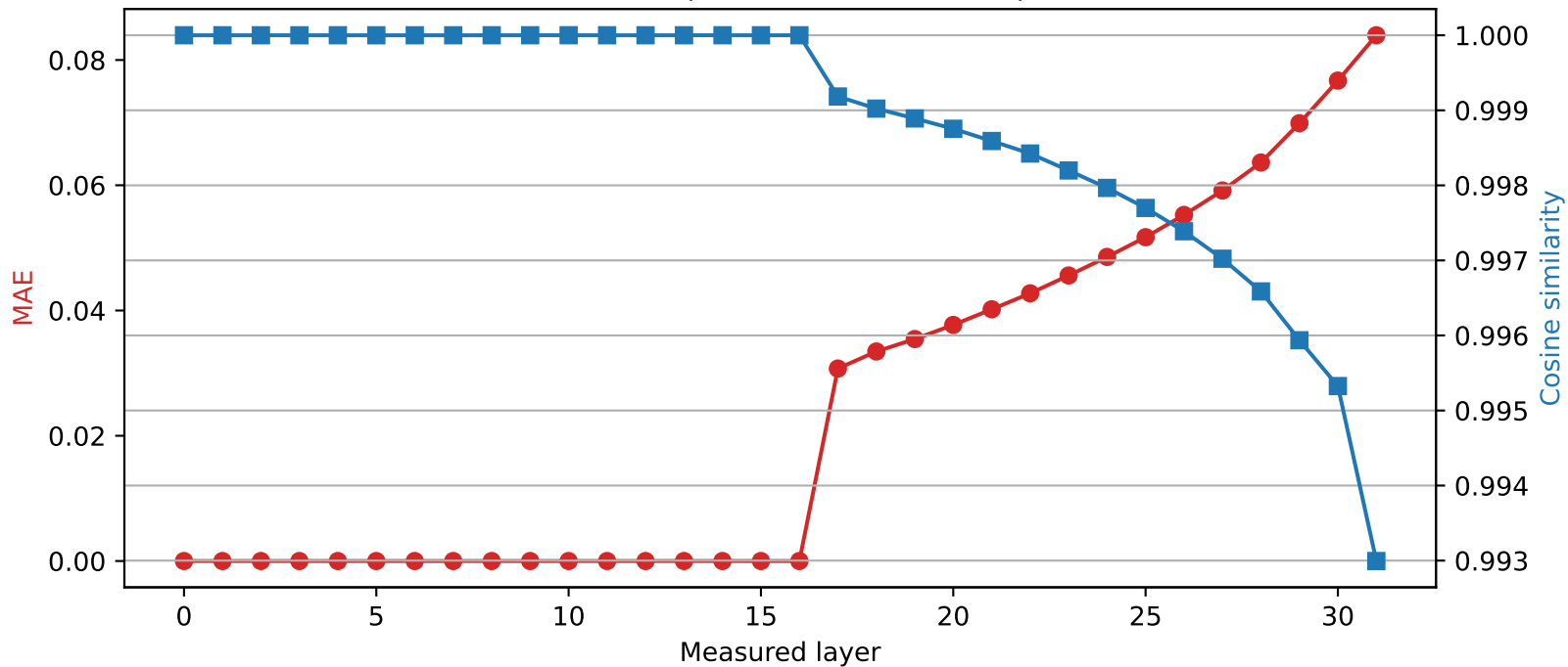
Mistral-7B-Instruct-v0.3 | Quantized layer 16 | float32 \rightarrow int2
