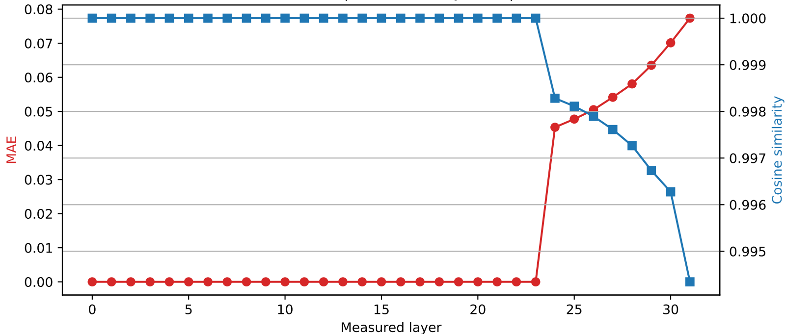
Mistral-7B-Instruct-v0.3 | Quantized layer 23 | float32 \rightarrow int2
