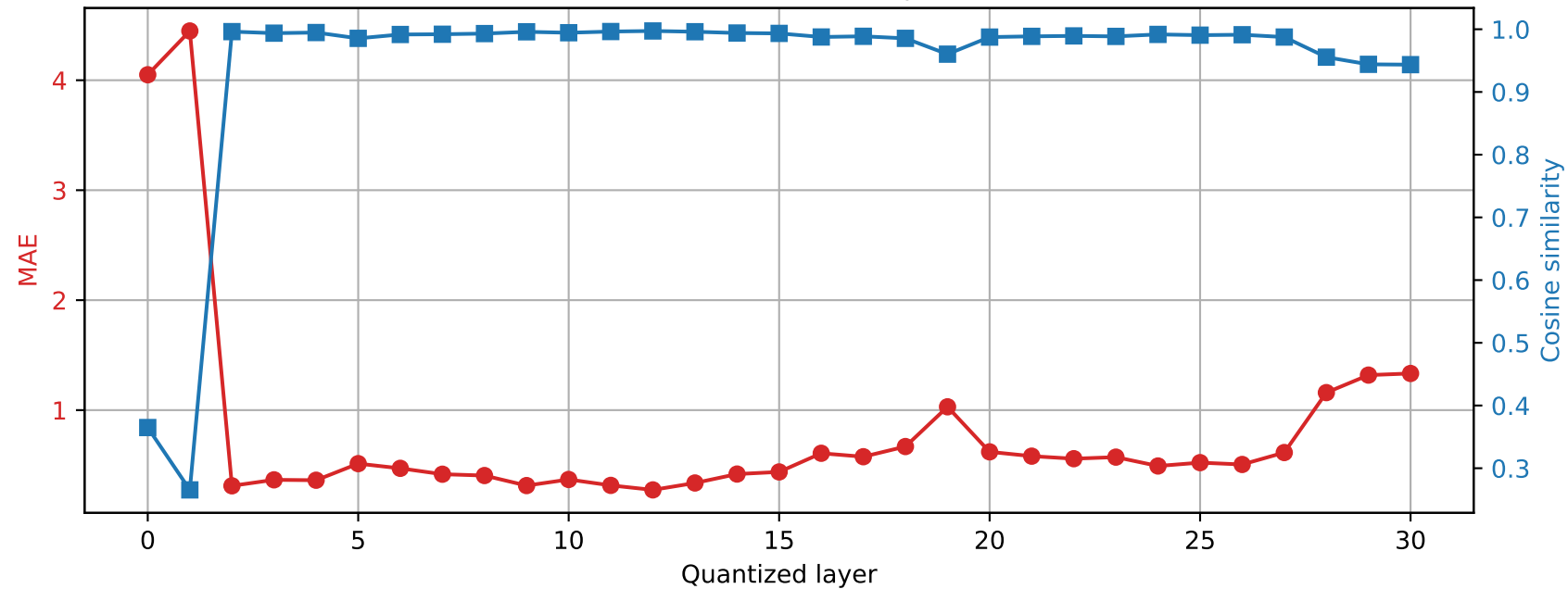
Mistral-7B-Instruct-v0.3 | Prompt 4 Final RMSNorm output damage | float32 \rightarrow int2
