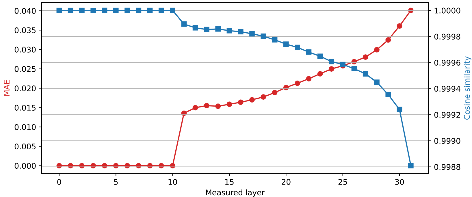
Mistral-7B-Instruct-v0.3 | Quantized layer 10 | float32 \rightarrow int2
