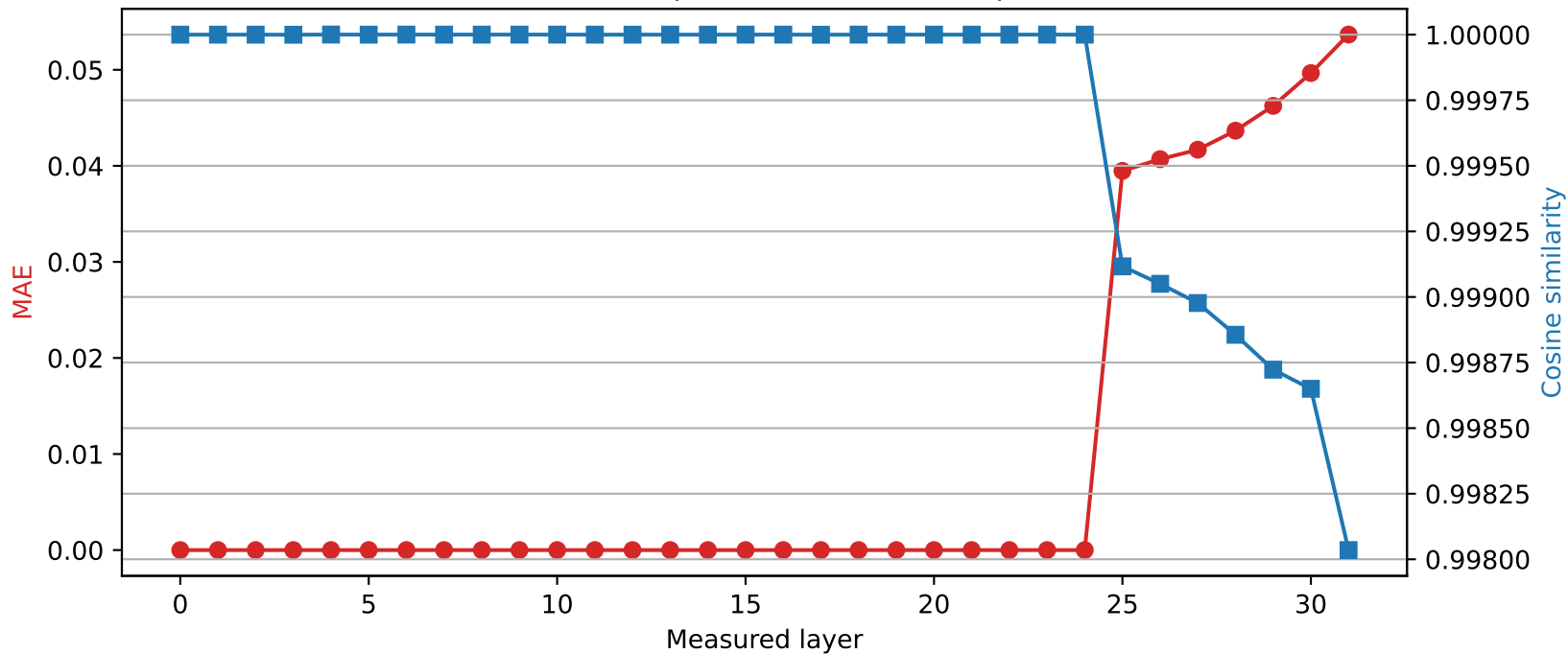
Mistral-7B-Instruct-v0.3 | Quantized layer 24 | float32 \rightarrow int2
