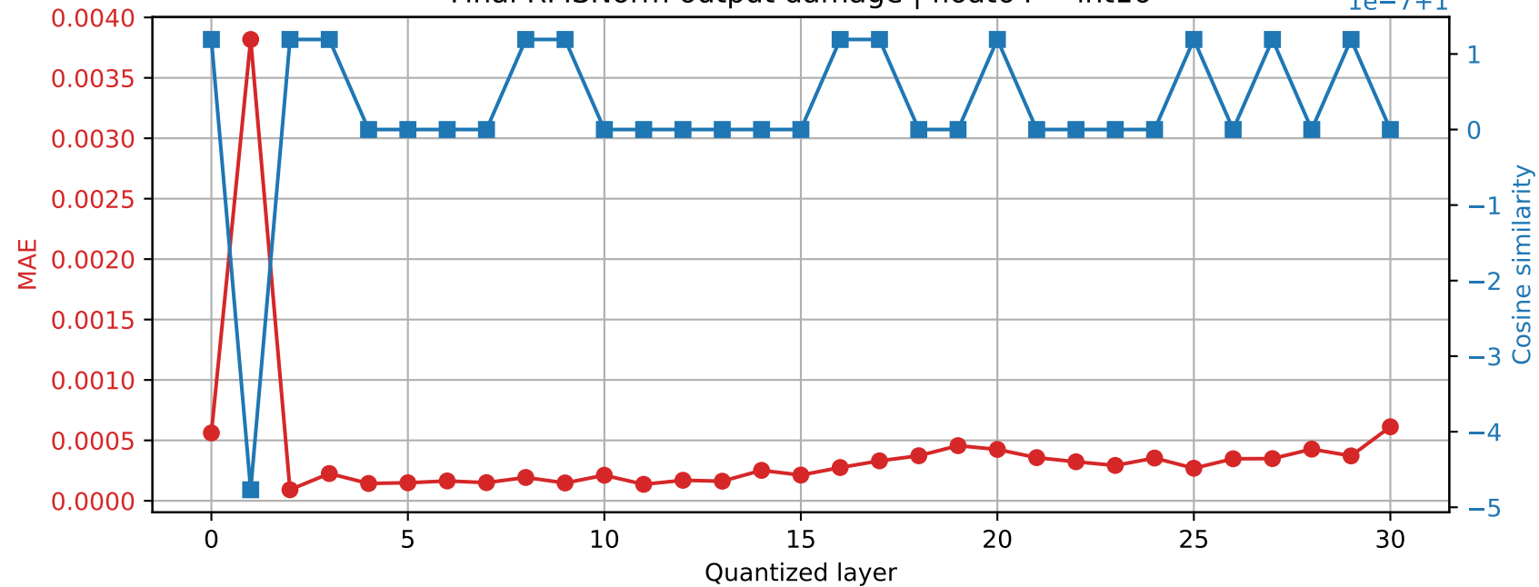
Mistral-7B-Instruct-v0.3 | Prompt 0 Final RMSNorm output damage | float64 \rightarrow int16
