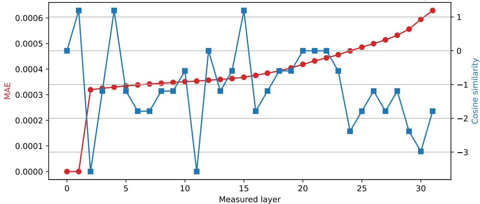
Mistral-7B-Instruct-v0.3 | Quantized layer 1 | float64 → int16
