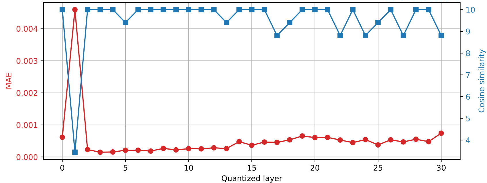
Mistral-7B-Instruct-v0.3 | Prompt 2 Final RMSNorm output damage | float64 → int16
