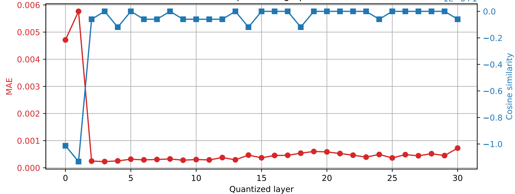
Mistral-7B-Instruct-v0.3 | Prompt 3 Final RMSNorm output damage | float64 → int16
