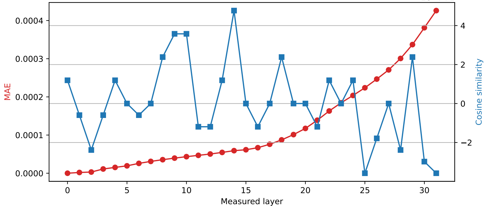
Mistral-7B-Instruct-v0.3 | Quantized layer 0 | float64 → int16
