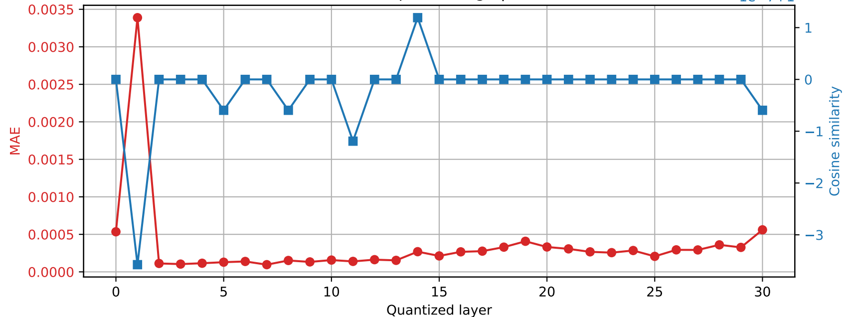
Mistral-7B-Instruct-v0.3 | Prompt 4 Final RMSNorm output damage | float64 → int16
