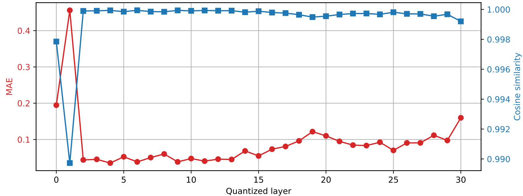
Mistral-7B-Instruct-v0.3 | Prompt 0 Final RMSNorm output damage | float64 \rightarrow int8
