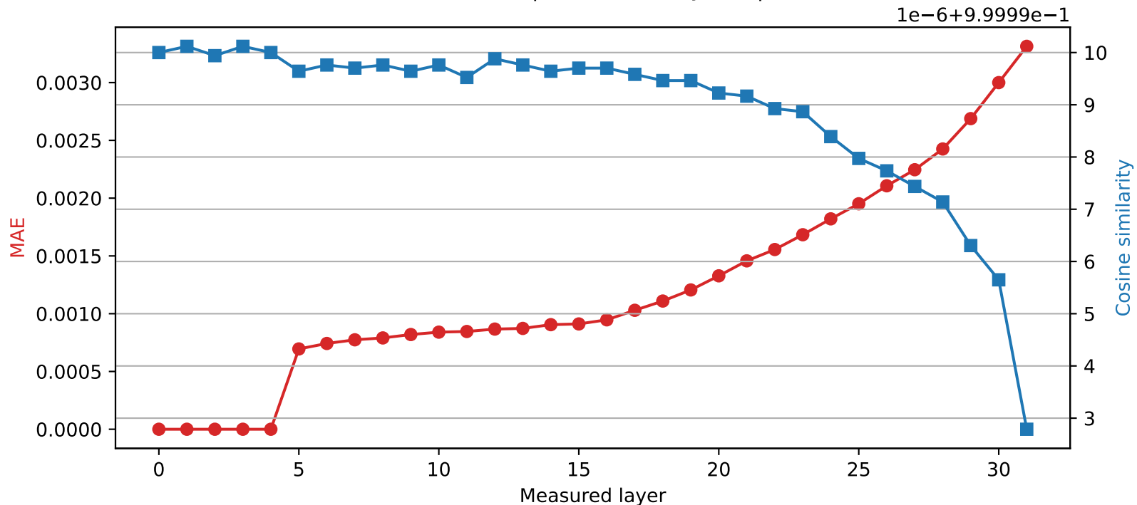
Mistral-7B-Instruct-v0.3 | Quantized layer 4 | float64 → int8
