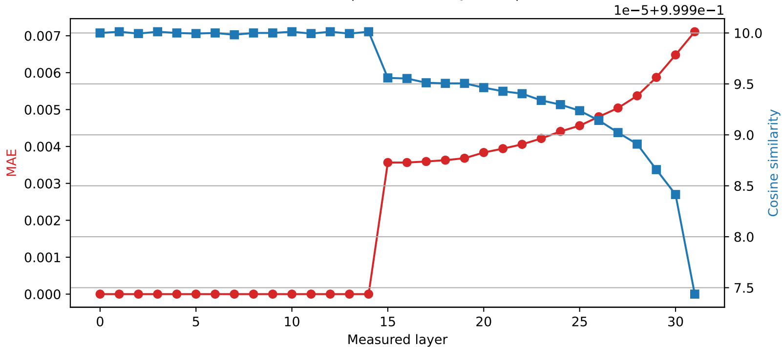
Mistral-7B-Instruct-v0.3 | Quantized layer 14 | float64 → int8
