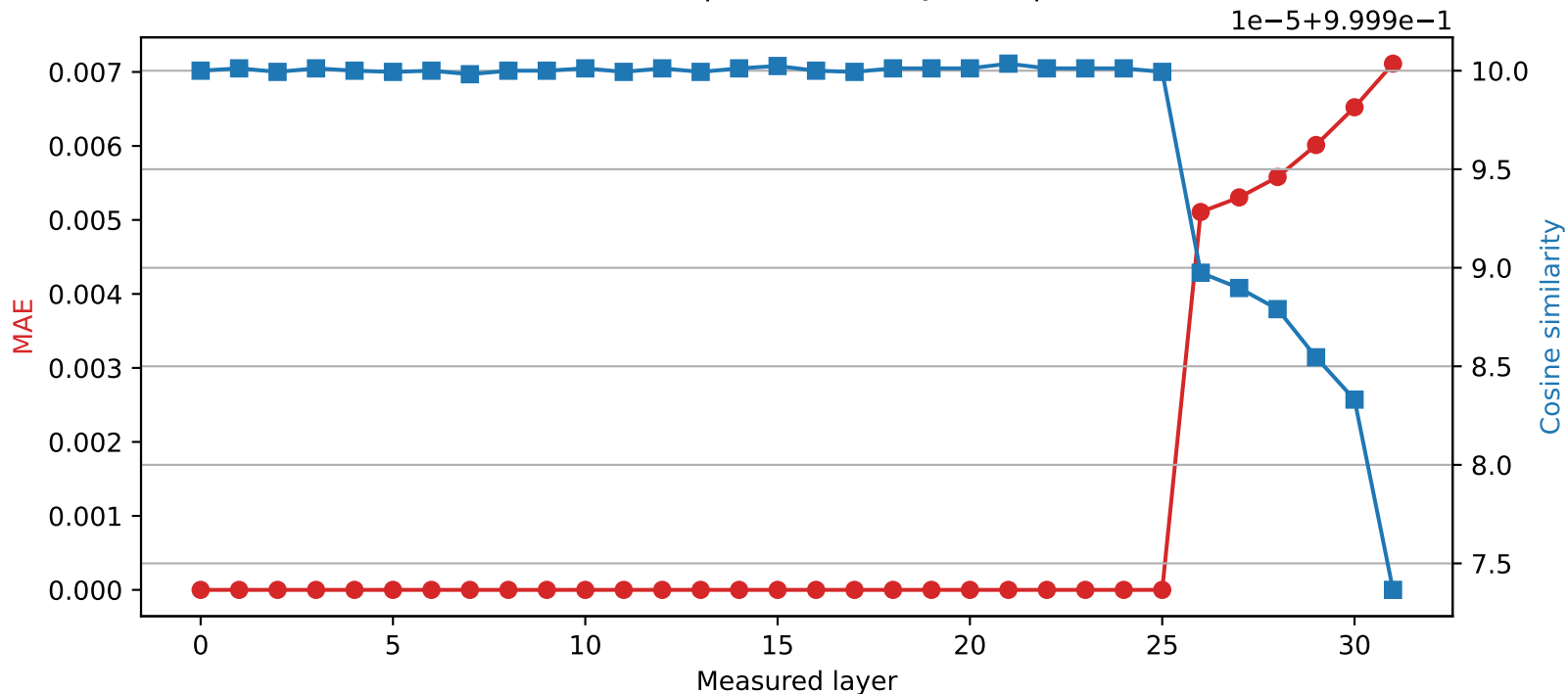
Mistral-7B-Instruct-v0.3 | Quantized layer 25 | float64 → int8
