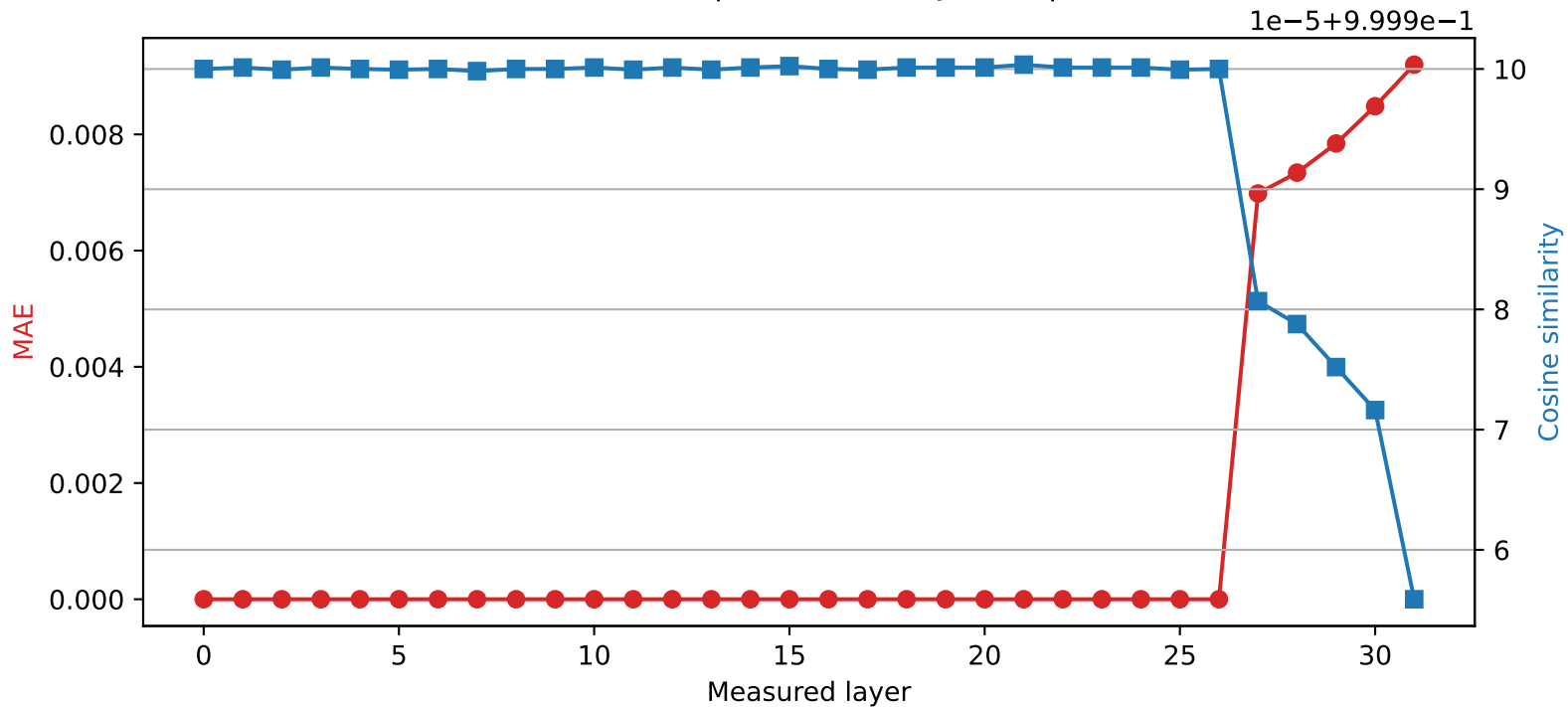
Mistral-7B-Instruct-v0.3 | Quantized layer 26 | float64 → int8
