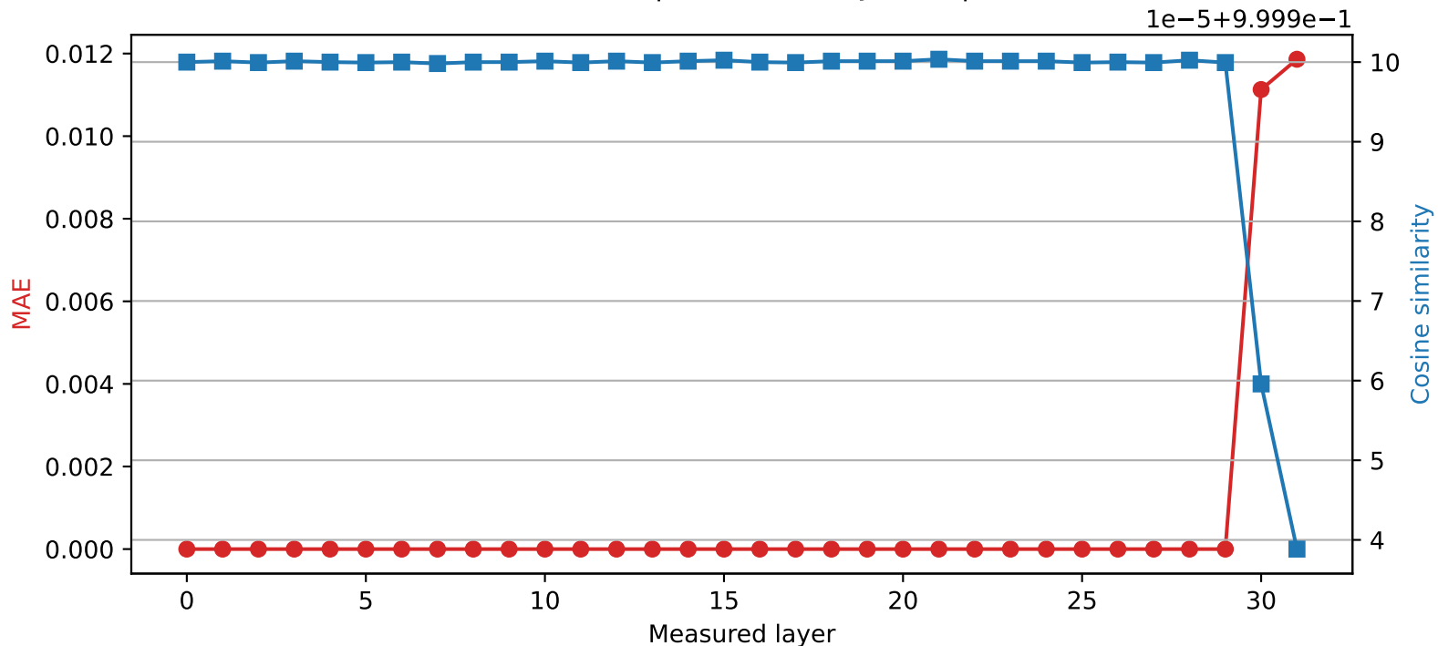
Mistral-7B-Instruct-v0.3 | Quantized layer 29 | float64 \rightarrow int8
