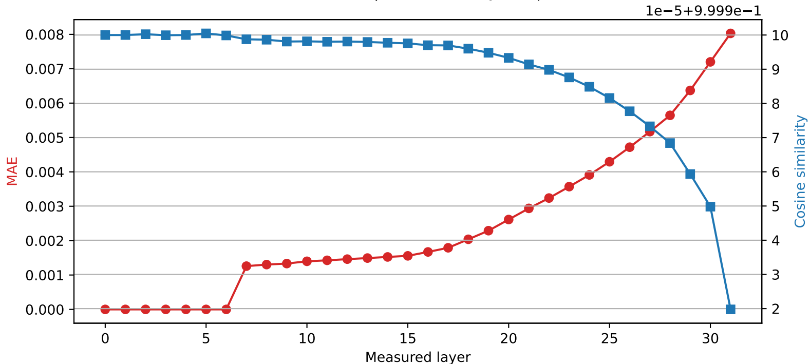
Mistral-7B-Instruct-v0.3 | Quantized layer 6 | float64 → int8
