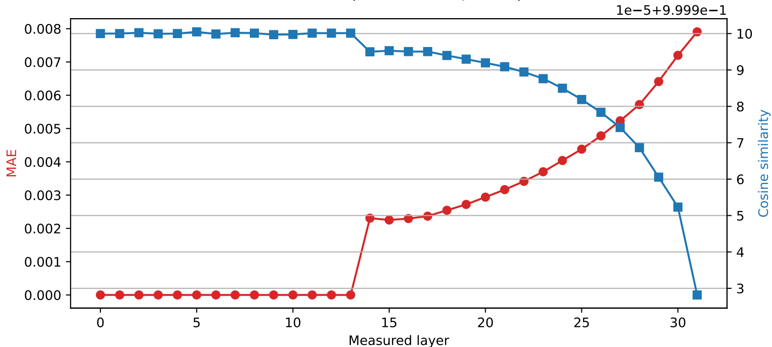
Mistral-7B-Instruct-v0.3 | Quantized layer 13 | float64 \rightarrow int8
