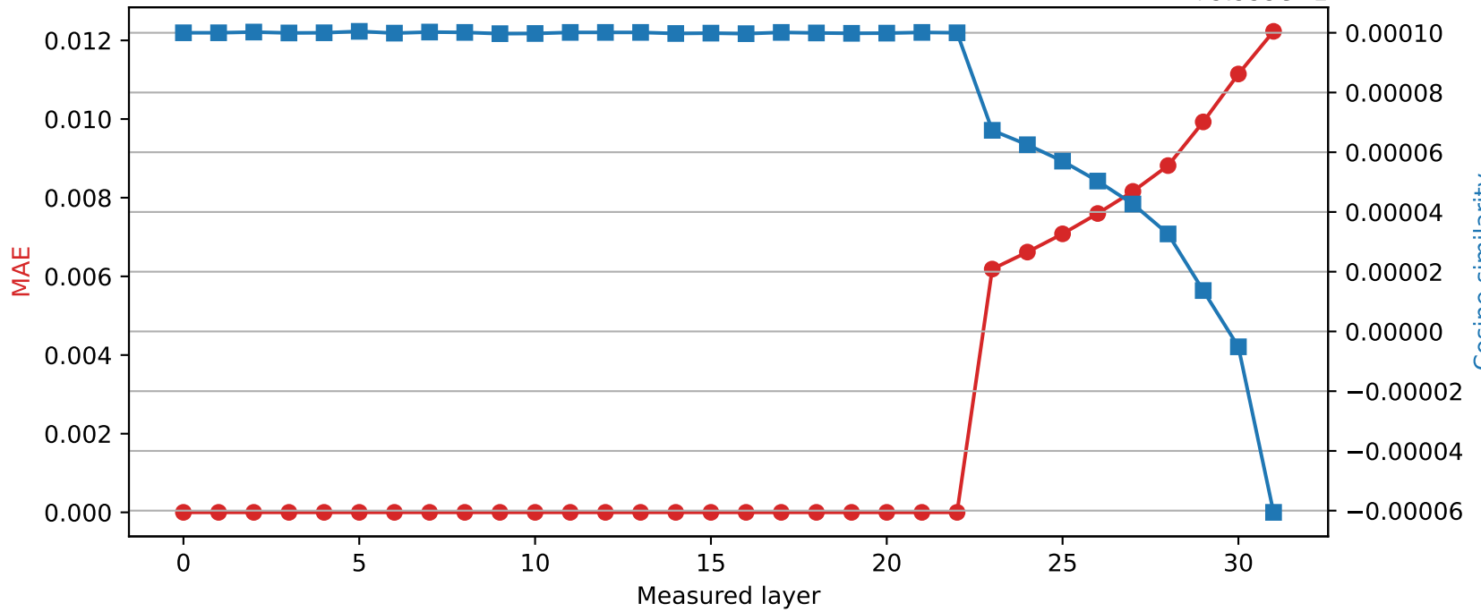
Mistral-7B-Instruct-v0.3 | Quantized layer 22 | float64 → int8 +9.999e-1
