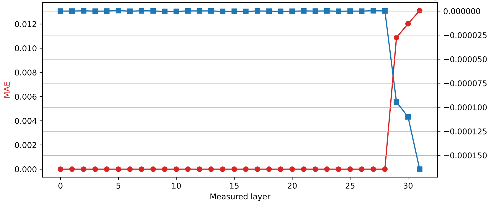
Mistral-7B-Instruct-v0.3 | Quantized layer 28 | float64 → int8
