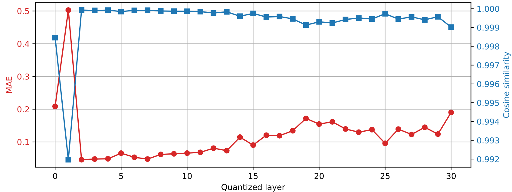
Mistral-7B-Instruct-v0.3 | Prompt 2 Final RMSNorm output damage | float64 → int8
