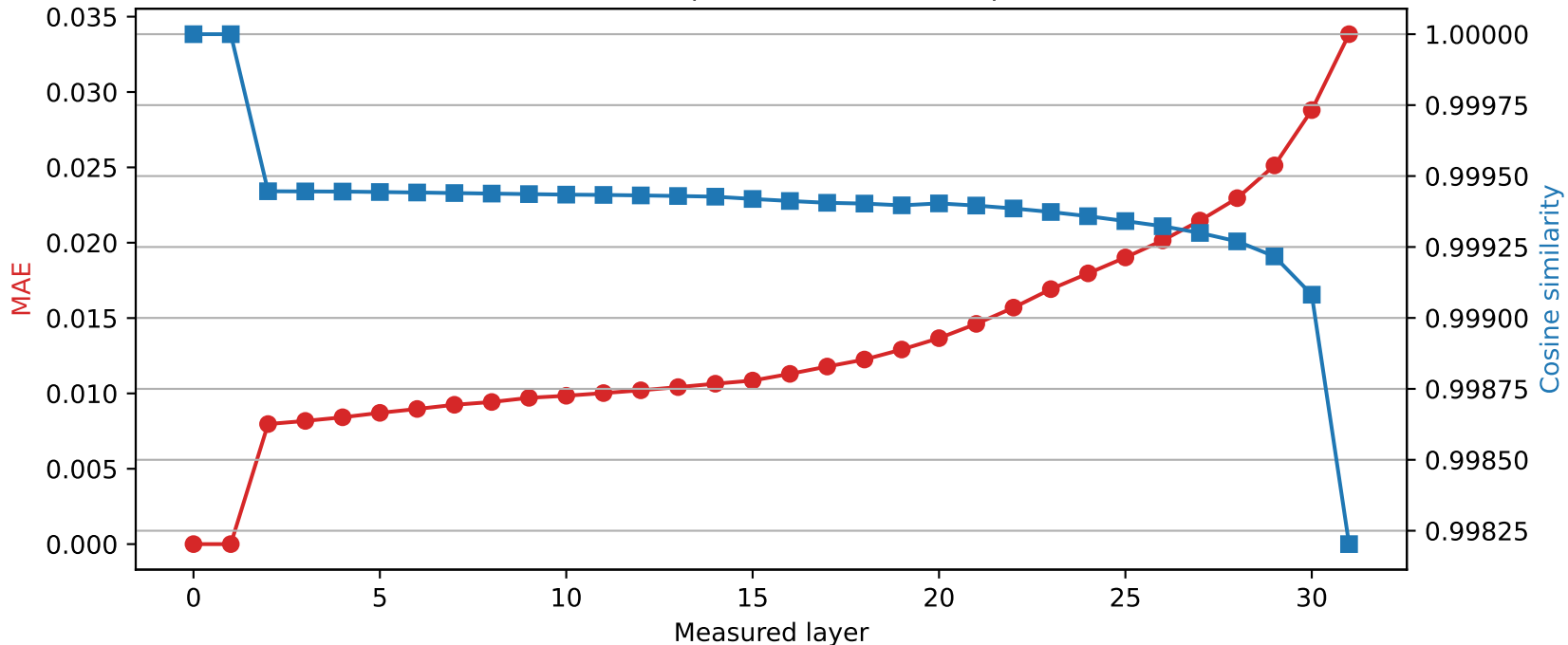
Mistral-7B-Instruct-v0.3 | Quantized layer 1 | float64 → int8
