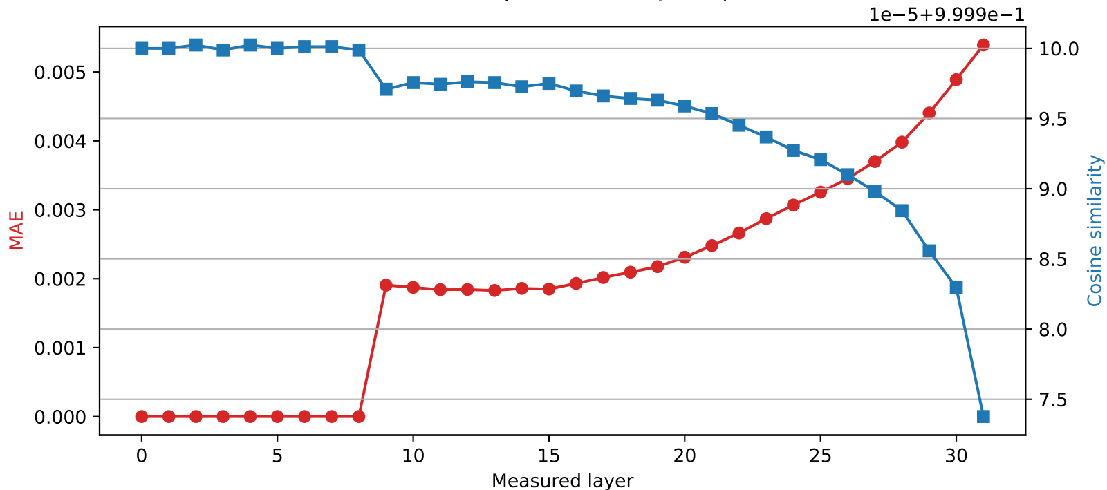
Mistral-7B-Instruct-v0.3 | Quantized layer 8 | float64 → int8
