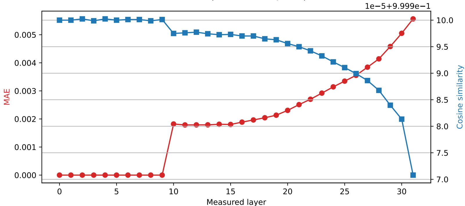
Mistral-7B-Instruct-v0.3 | Quantized layer 9 | float64 → int8
