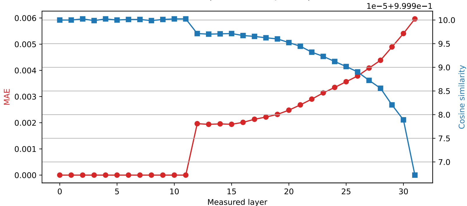
Mistral-7B-Instruct-v0.3 | Quantized layer 11 | float64 → int8
