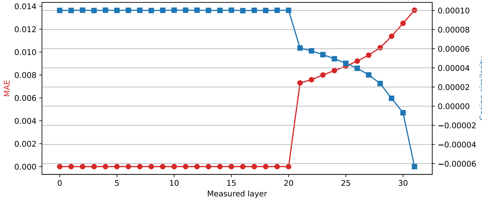
Mistral-7B-Instruct-v0.3 | Quantized layer 20 | float64 \rightarrow int8 +9.999e-1
