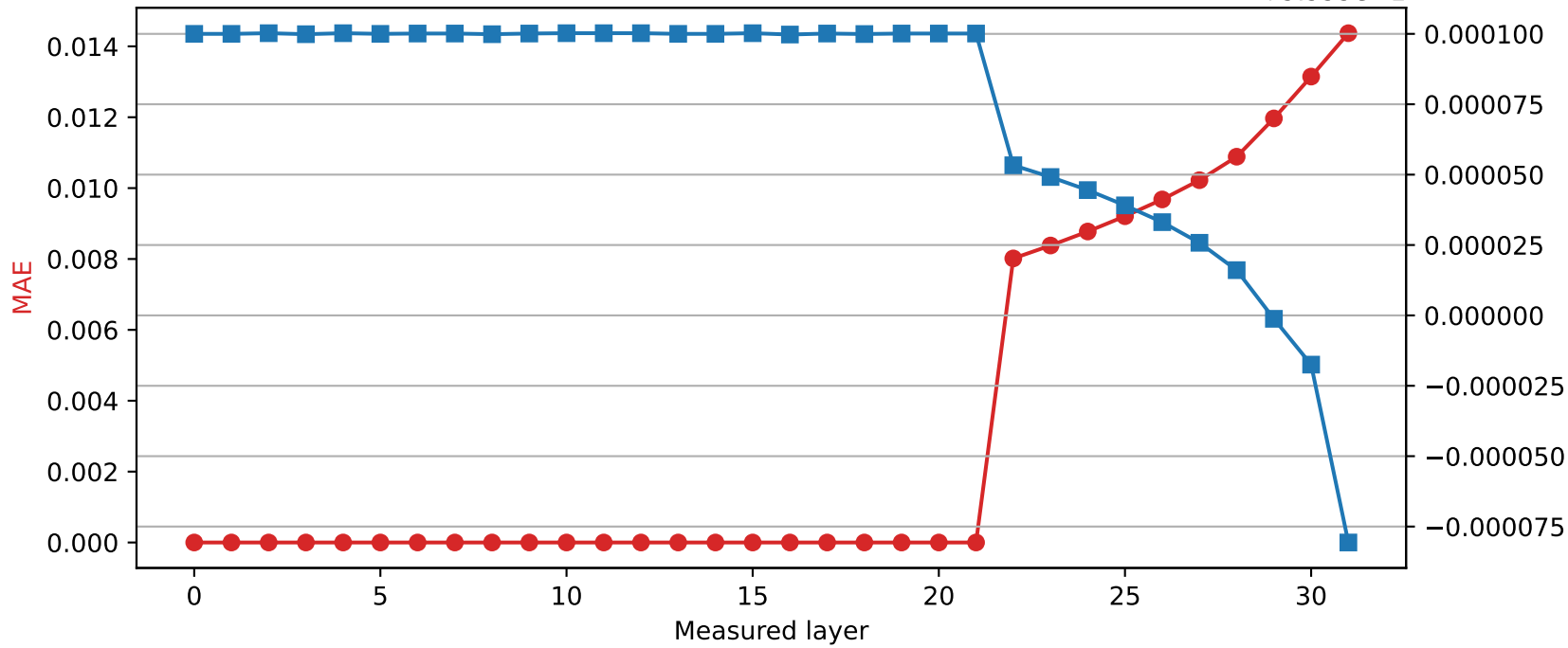
Mistral-7B-Instruct-v0.3 | Quantized layer 21 | float64 \rightarrow int8 +9.999e-1
